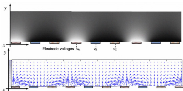
FIGURE 4. Electrodynamic screen [64].
