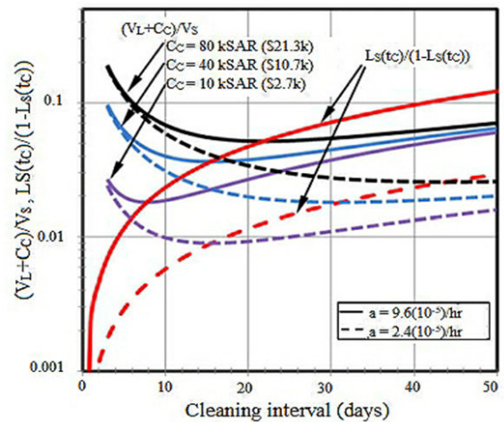
FIGURE 10. Cleaning interval based on Cost of Energy (CoE) [82].
