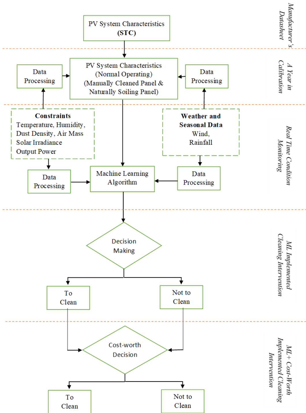
FIGURE 12. Suggested model for scheduling the cleaning intervention.
