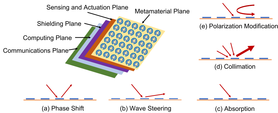
FIGURE 4. Conceptual design of a plasmonic reflectarray able to unconventionally manipulate EM waves [48].
