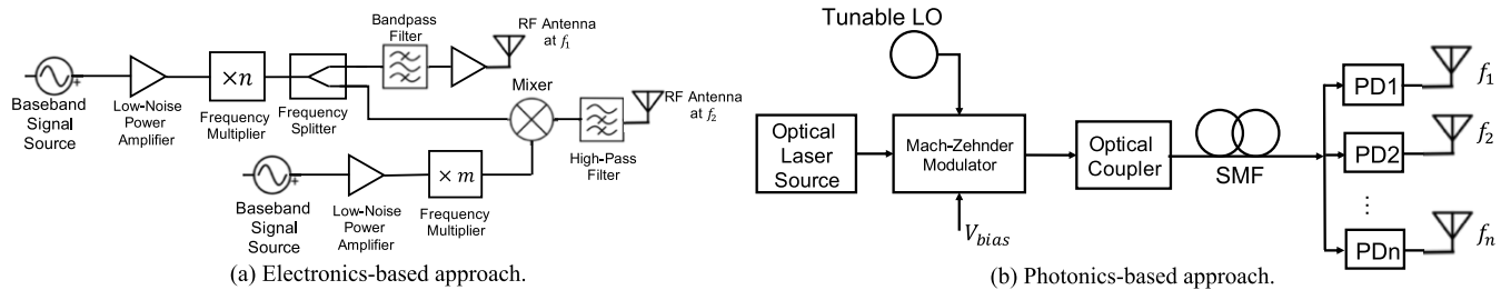
FIGURE 12. The proposed all-spectrum signal front-end designs [141].
