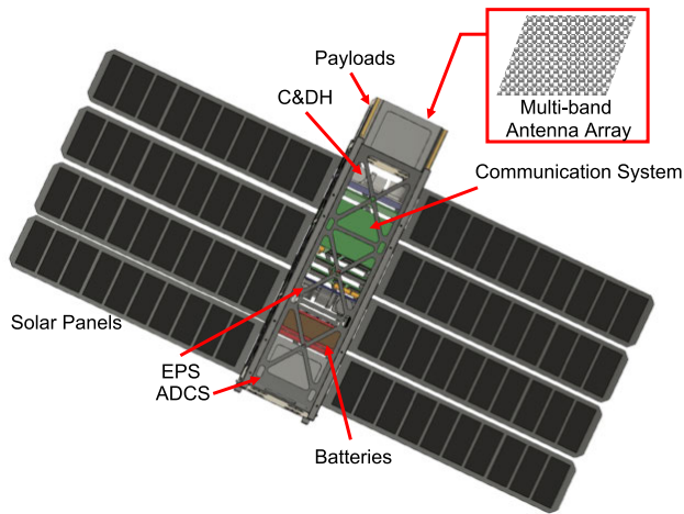
FIGURE 11. Conceptual design of a next-generation CubeSat [141].
