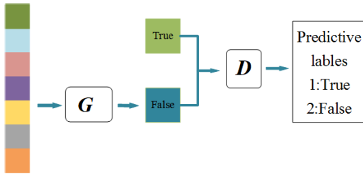
FIGURE 14. The model of GAN. The main functions of G and D are presented as follows. G is a generative network, which receives a random noise z and generates an image through this noise. D is a discrimination network, which judges whether a picture is “real”. Its input parameter is x , which represents a picture, and the output D(x) represents the probability that x is a real picture. If it is 1, it represents 100% of the real picture. If it is 0, which represents the impossible picture.
