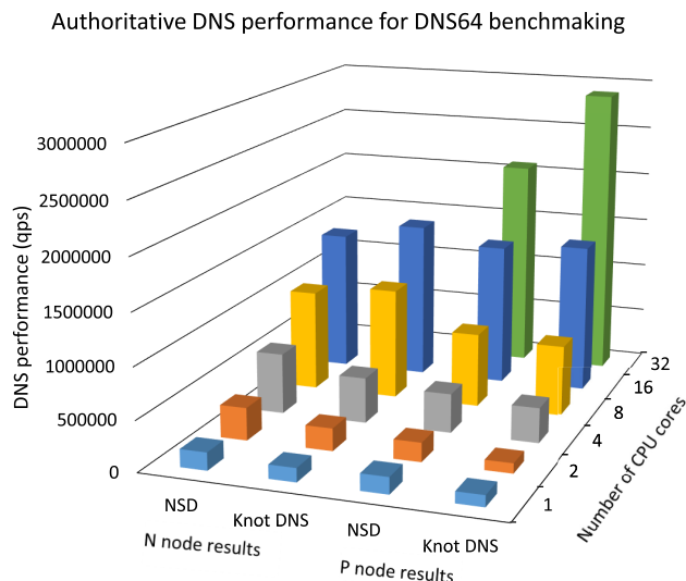
FIGURE 4. Comparison of NSD and Knot DNS for DNS64 benchmarking. (The N node result of Knot DNS at 16 cores is limited by Tester performance.)
