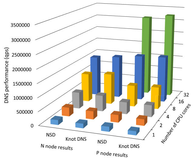
FIGURE 3. Comparison of NSD and Knot DNS for DNS server operation. (The N node result of Knot DNS at 16 cores is limited by Tester performance.)
