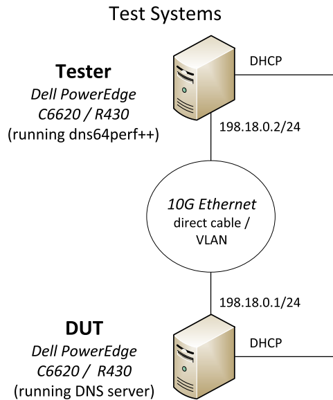
FIGURE 2. Measurement setup for all types of measurements.
