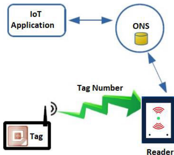
FIGURE 4. RFID operation.
