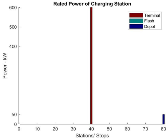
FIGURE 8. Charger deployment for Route C.
