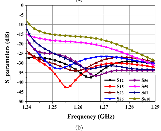
FIGURE 14. S-parameters of the 4 × 4 antenna with DSSA. (a) Top view of the geometry. (b) Typical scattering parameters.
