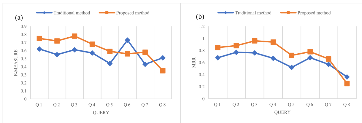
FIGURE 10. F-score and (b) MRR experimental results.
