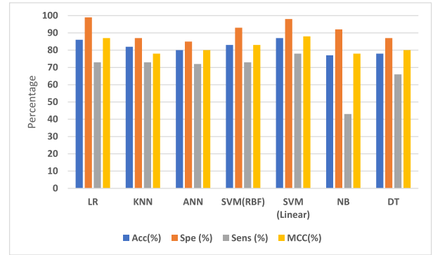
FIGURE 9. Classifiers performances on 6 important features selected set by mRMR.
