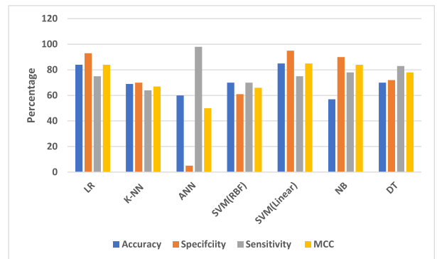
FIGURE 7. Classifiers performance with LOSO CV on set of full features.
