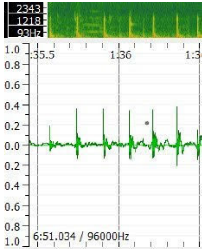
FIGURE 2. An example of spectrogram and time-series representation of Bryde's whale pulse call. The sound was recorded in Gordon's bay harbour, False bay, South-West, South Africa [52].
