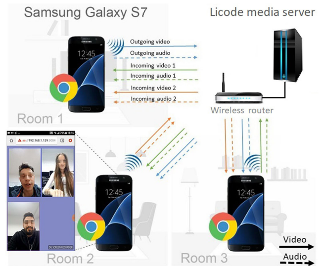
FIGURE 9. Testbed set-up over a LAN connection (User Study 5).
