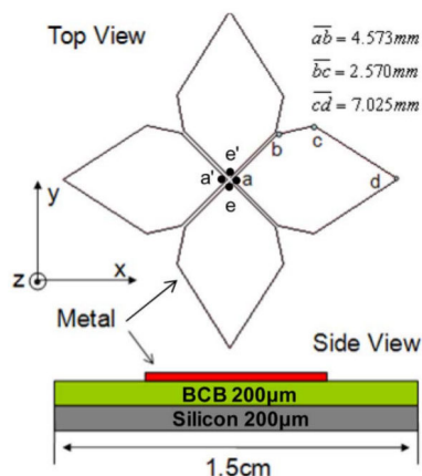
FIGURE 13. Geometry of the fourtear antenna presented in [92] (©[2008] IEEE).
