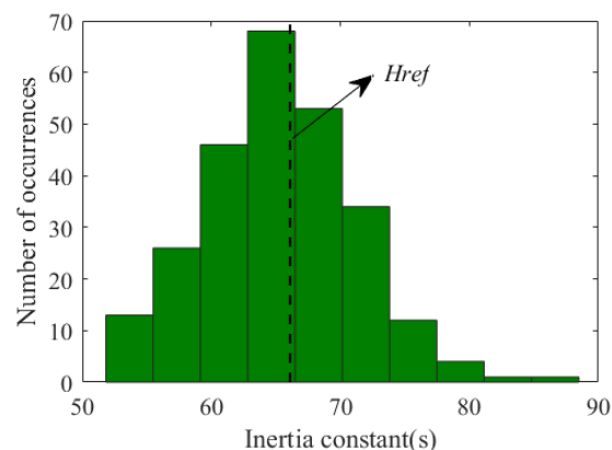
FIGURE 8. Distribution of the estimated inertia constant of area 2.
