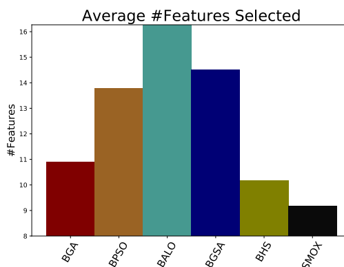
FIGURE 9. Average number of features selected by the proposed SMOX algorithm and five classic meta-heuristic methods over 18 UCI datasets.
