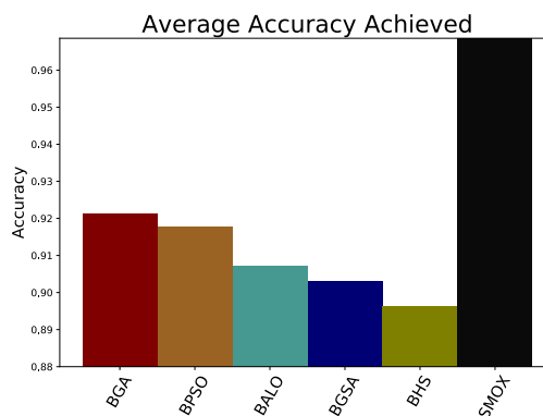
FIGURE 8. Average accuracies achieved by the proposed SMOX algorithm and five classic meta-heuristic methods over 18 UCI datasets.
