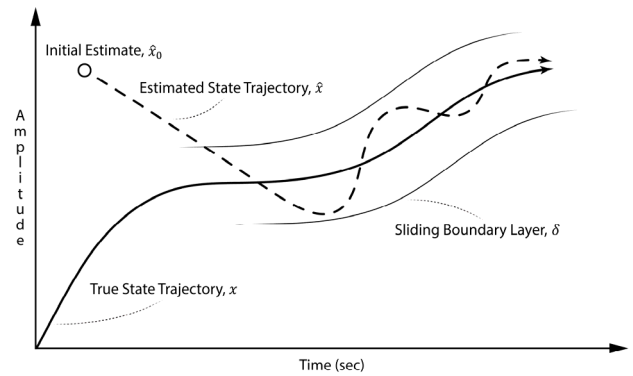
FIGURE 1. The sliding innovation filter (SIF) concept illustrating the effects of the switching gain and sliding boundary layer.
