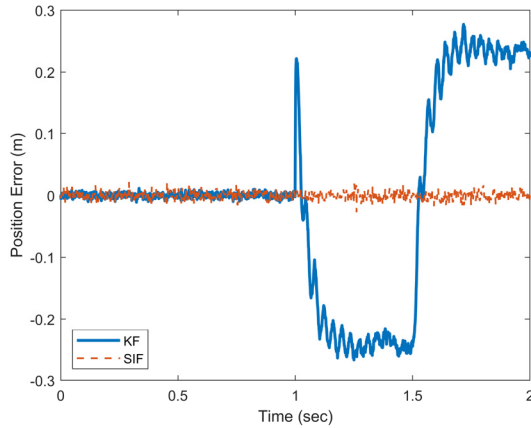
FIGURE 5. Position estimation error for the KF and SIF for the linear EHA faulty case. This further illustrates the robustness of the SIF gain.
