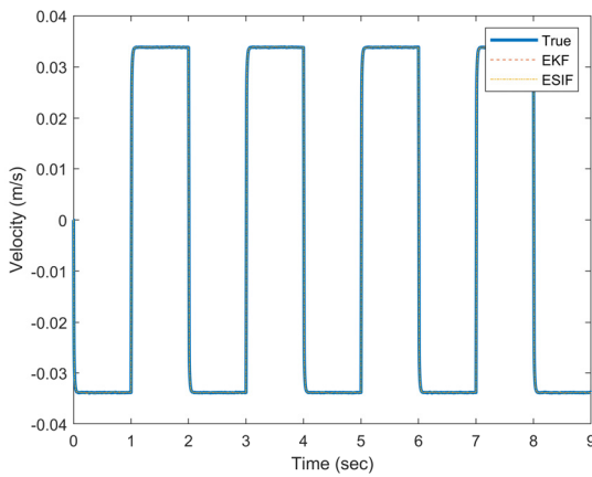
FIGURE 7. EHA velocity trajectory and corresponding EKF and ESIF estimates. Note that the results are nearly identical, so appear to be over-lapping.
