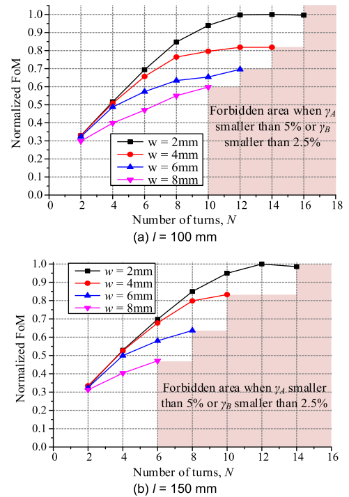
FIGURE 19. Normalized figure of merit (FoM) plot for two cases.
