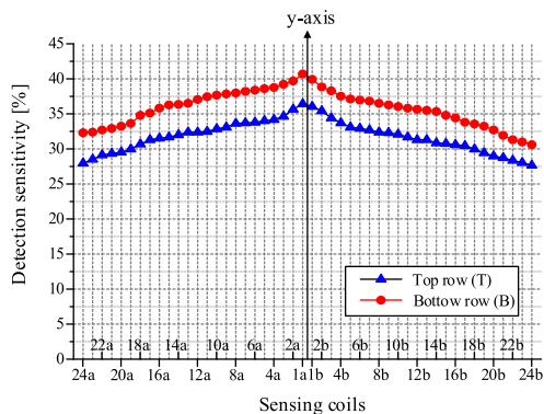
FIGURE 23. Symmetric detection sensitivity of two sensing coils a and b of each channel: top row channels from T1 to T24 (triangle symbol), and bottom row channels from B1 to B24 (circle symbol).
