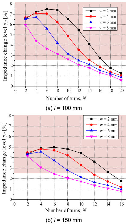
FIGURE 18. Impedance change level \gamma_B with various values of w and N with the metal object between two adjacent sensing coils.
