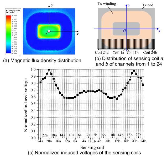
FIGURE 3. FEM simulation showing the symmetrical distribution about the y-axis of the z-direction magnetic flux density generated by the Tx coil current.
