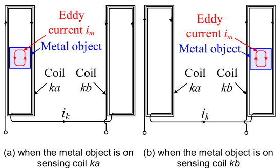
FIGURE 4. Two cases of when a metal object is on only one sensing coil of channel k .
