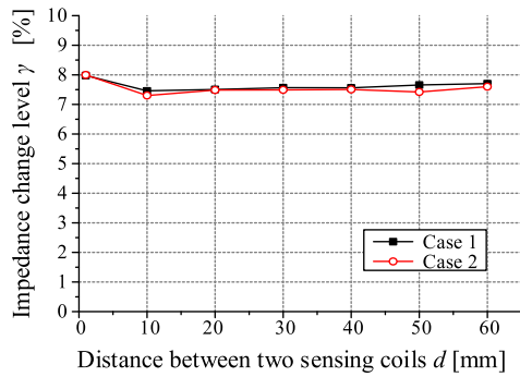
FIGURE 11. FEM simulation results in two cases of Figure 10.
