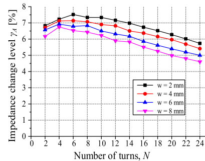
(a) l = 100 mm
