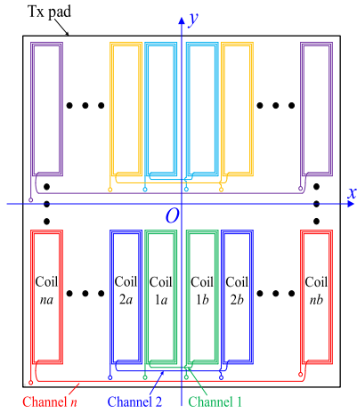
FIGURE 2. Conceptual design of the proposed symmetric sensing coil. Channels are differentiated by the different colors. Each channel includes two sensing coils, which have same number of turns and which are shown in the same color.
