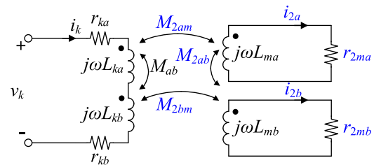
(b) with respect to eddy current i_2
