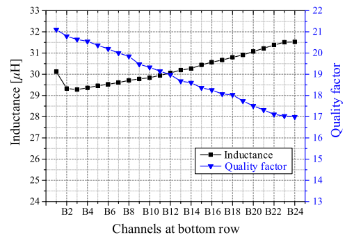
(b) Channels at bottom row: from B1 to B24
