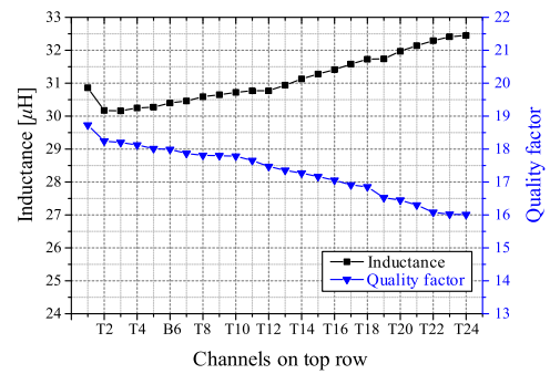
(a) Channels on top row: from T1 to T24
