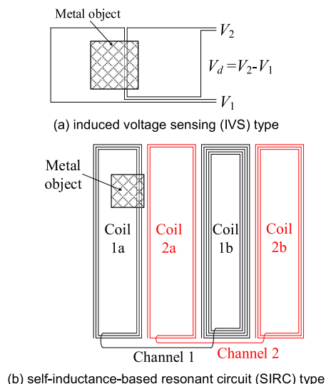
FIGURE 1. Conventional MOD methods of magnetic field change sensing (MFCS).
