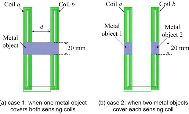
FIGURE 10. Two cases of when the metal object is on both two sensing coils of channel k .
