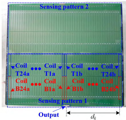
(a) Proposed symmetric sensing patterns. Each sensing pattern includes 48 channels and two rows, covering half of the Tx pad.
