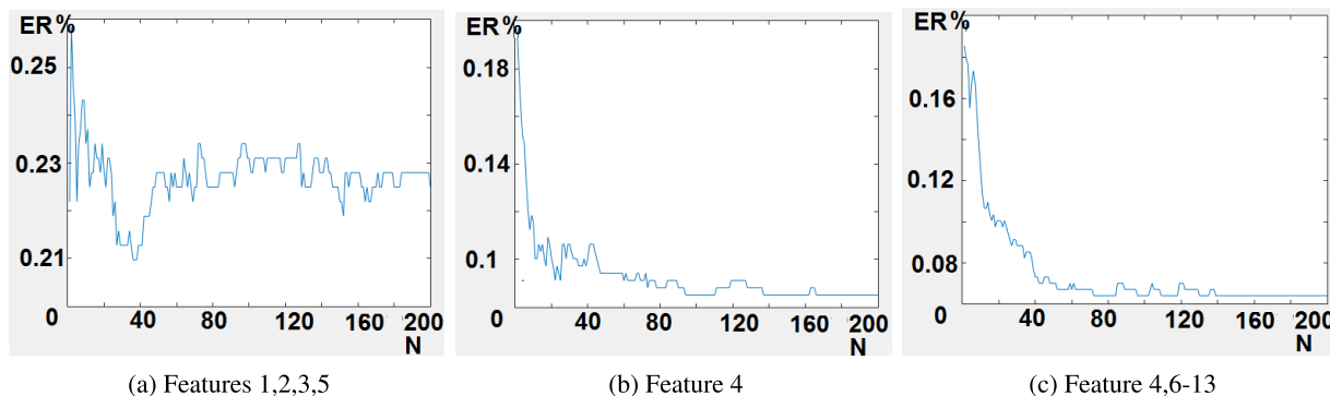
FIGURE 7. Effect of The selected features on classification error, (N = number of decision trees), (ER% = error rate), (1 = count of piece of Arabic words (PAWs), 2 = number of holes), (3 = eccentricity), (4 = extent), (5 = orientation with x-axis), (6-13 = eight geometric features).
