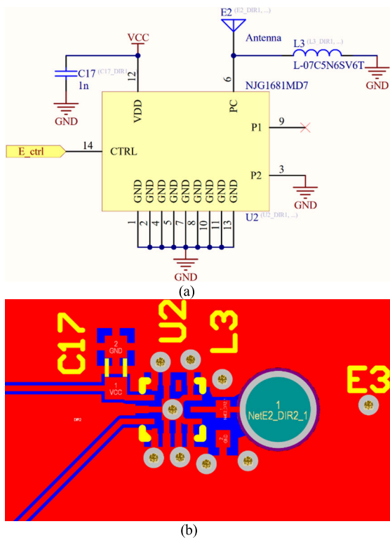
FIGURE 5. SPDT switching circuit model – a) electric scheme, b) layout.
