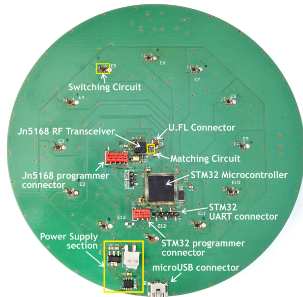
FIGURE 6. Components placement on the bottom of the WSN node.
