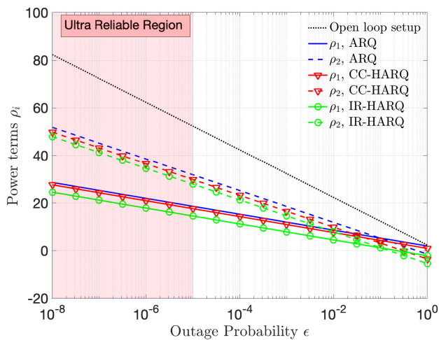
FIGURE 5. Transmit power in each round to achieve a target outage probability for rate R = 1 npcu.
