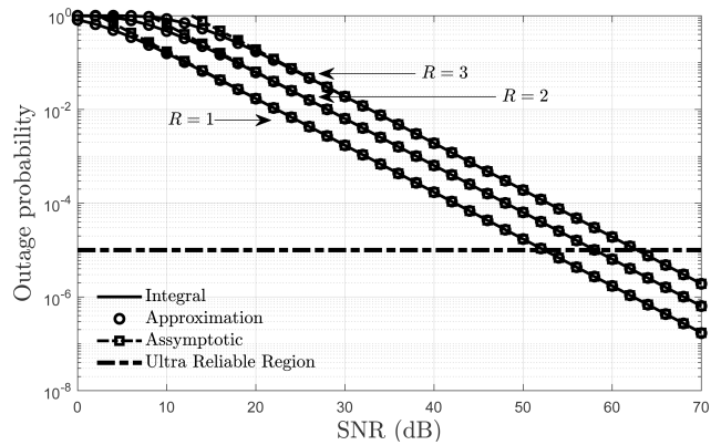
FIGURE 1. Outage probability for the open loop setup for different channel coding rates.
