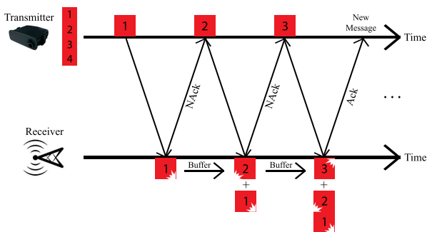
FIGURE 4. The setup for IR-HARQ protocol. The transmitter splits the message into several packets. It sends first packet 1 and waits for reply from the receiver. If it receives NACK packet, then it sends more redundancy through packet 2 and so on. Meanwhile, the receiver buffers the packets and combines them to extract the information.
