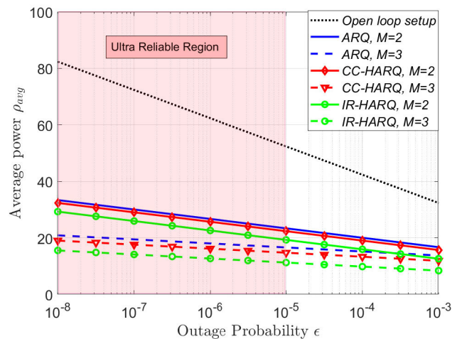
FIGURE 7. Average power required to achieve a target outage probability for rate R = 1 npcu when the maximum number of transmissions is fixed to M = 2 and M = 3 .
