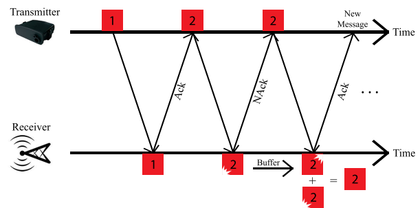
FIGURE 3. The setup for CC-HARQ protocol. The transmitter sends first packet 1 and waits for the ACK from the receiver. Then it sends packet 2. If the receiver can not decode the packet, it buffers the packet and asks for retransmission. Then, when it receives packet 2 once more, it combines it with the buffered packet to extract the information.
