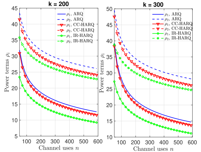
FIGURE 6. Power terms as a function of the number of channel uses for different number of information nats.
