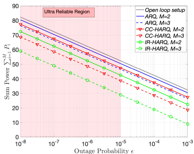
FIGURE 8. Maximum power that will be spent to achieve a target outage probability for rate R = 1 npcu when the maximum number of transmissions is fixed to M = 2 and M = 3 .
