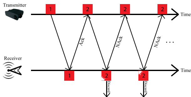
FIGURE 2. The setup for ARQ protocol. The transmitter sends the first packet and waits for the ACK from the receiver. Then it sends packet 2. If the receiver can not decode the packet, it discards the packet and asks for retransmission.
