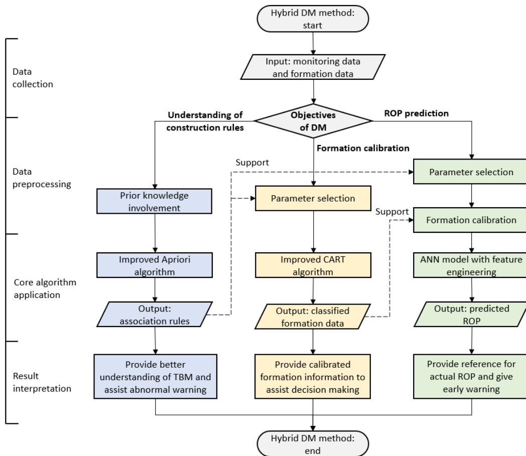
FIGURE 1. Framework of the hybrid DM method.
