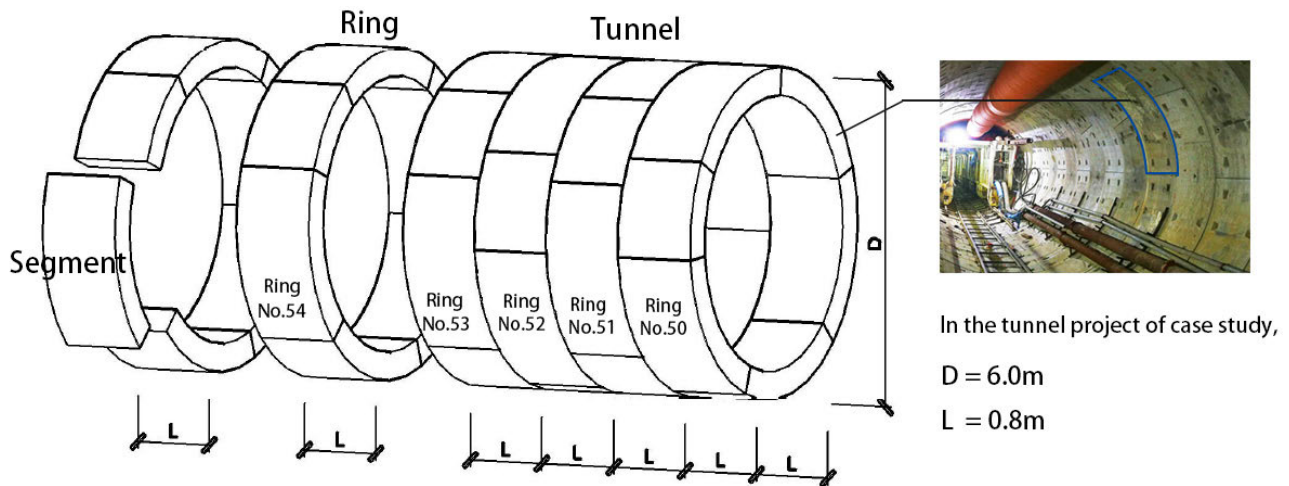
FIGURE 3. Ring in tunnel construction.
