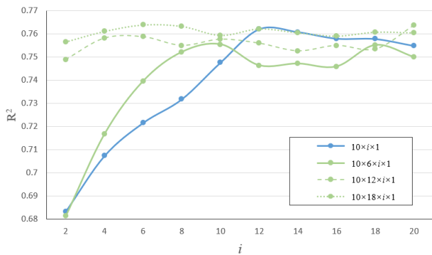
FIGURE 10. Model structure selection of BP neural network.
