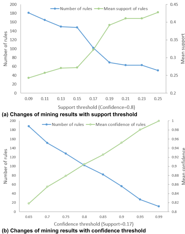
FIGURE 8. Parameter selection of Apriori algorithm.
