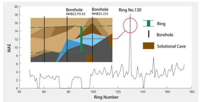
FIGURE 11. Prediction error of ROP for each tunnel ring.
