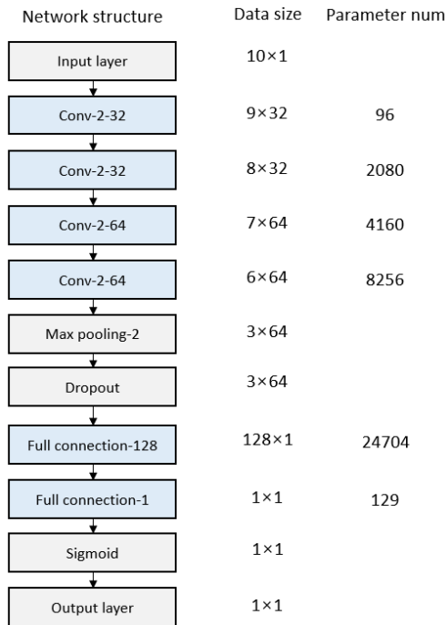
FIGURE 5. Structure of the CNN model.
