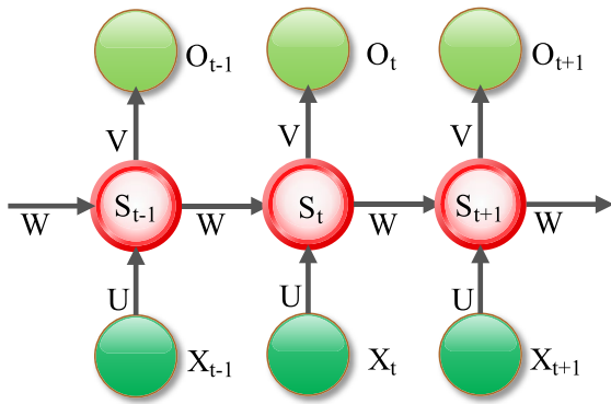
FIGURE 11. A typical RNN architecture.
