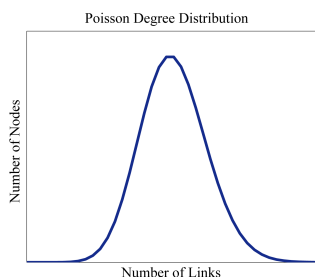
FIGURE 4. Poisson degree distribution.
