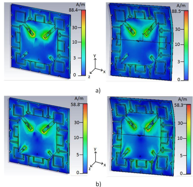
FIGURE 9. Amplitude of surface current distribution for planar and bent form at (a) 1.575 GHz and (b) 2.45 GHz.
