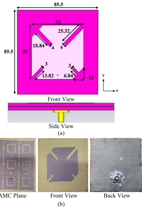
FIGURE 3. Antenna design (a) topology of the dual-polarized planar textile antenna (all dimensions in mm) and (b) fabricated prototype.
