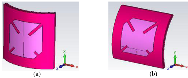
FIGURE 7. The antenna when bent at the (a) y -axis and (b) x -axis.
