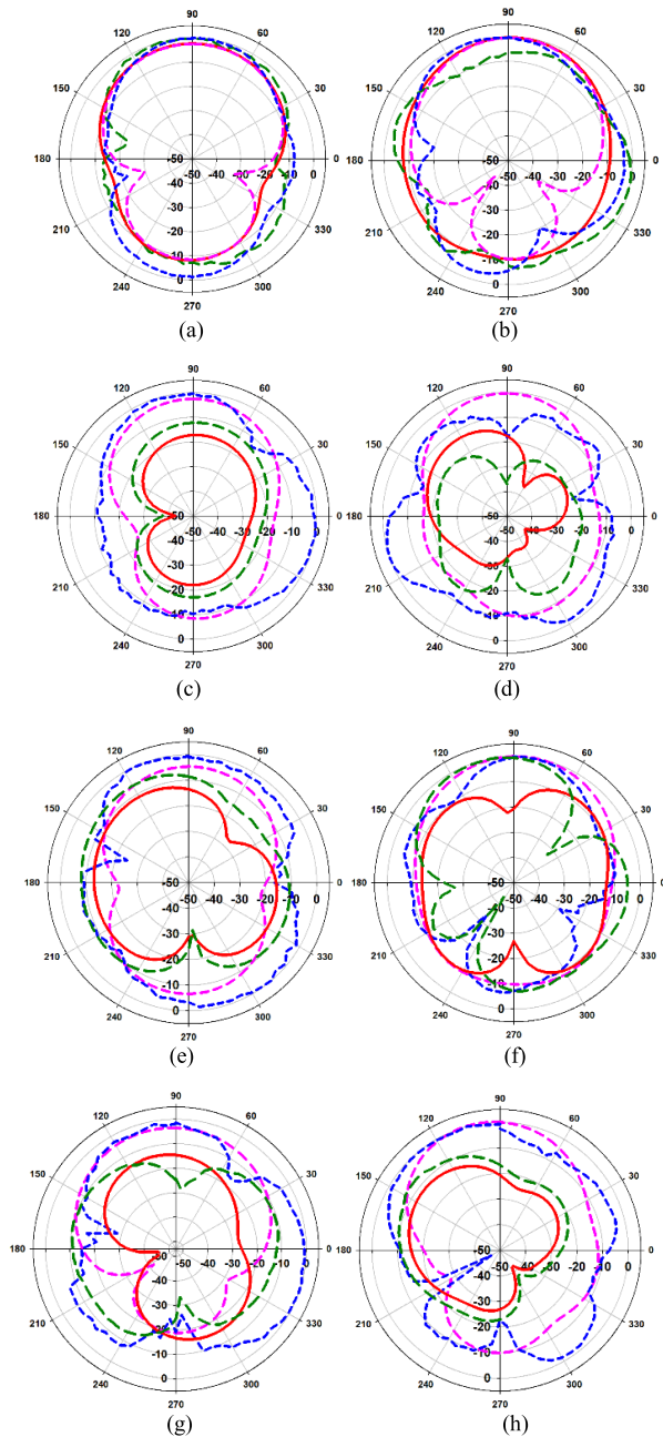
FIGURE 10. Simulated and measured radiation patterns of the proposed antenna when bent at the (a) x-axis (xz-plane) at 1.575 GHz, (b) x-axis (xz-plane at 2.45 GHz), (c) x-axis (yz-plane) at 1.575 GHz, (d) x-axis (yz-plane) at 2.45 GHz, (e) the y-axis (xz-plane) at 1.575 GHz, (f) the y-axis (xz-plane) at 2.45 GHz, (g) y-axis (yz-plane) at 1.575 GHz and (h) y-axis (yz-plane) at 2.45 GHz. Legend: simulated co-polarization (medium dashed pink line); simulated cross-polarization (solid red line); measured co-polarization (short dashed blue line); measured cross-polarization (long dashed dark green line).
