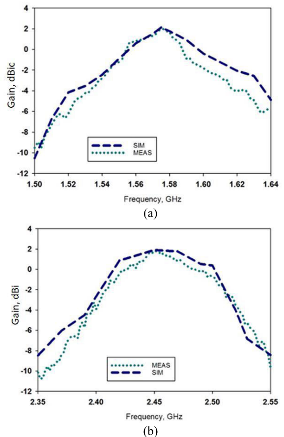
FIGURE 6. Simulated and measured realized gain across two frequency ranges when the antenna is in free space (a) lower band frequency (1.575 GHz) and (b) upper band frequency (2.45 GHz).
