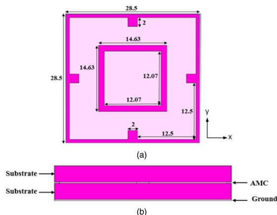
FIGURE 1. AMC unit cell (a) Dimensions of the AMC unit cell (in mm) and (b) AMC unit cell cross section with a substrate thickness of 2.64 mm per layer and conductor (AMC and ground) thickness of 0.17 mm per layer.
