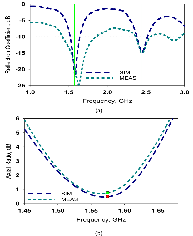
FIGURE 5. Simulated and measured results of the antenna performance: (a) reflection coefficient; and (b) axial ratio.
