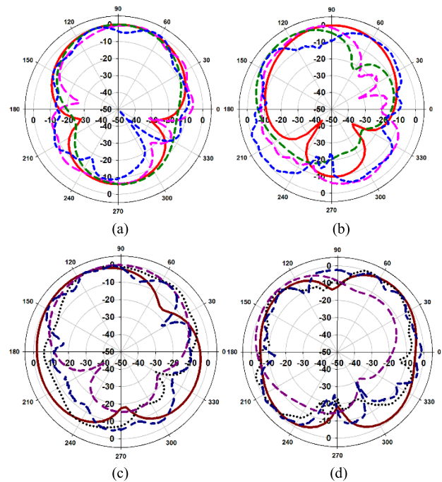
FIGURE 11. Simulated and measured radiation patterns at the yz-plane when the antenna is placed on the upper arm and shoulder at (a) 1.575 GHz bent at the x-axis, (b) 2.45 GHz bent at the x-axis, (c) 1.575 GHz bent at the y-axis and (d) 2.45 GHz bent at the y-axis. Legend: Simulation and measurement at the upper arm when bent on x-axis (solid red line and long dashed pink, respectively) and on the shoulder when bent at the x-axis (medium dash dark green and short dash blue, respectively); Simulation and measurement at the upper arm when bent on y-axis (solid dark red line and dotted black, respectively) and on the shoulder when bent at the y-axis (medium-medium dark pink and long-short dark blue, respectively).
