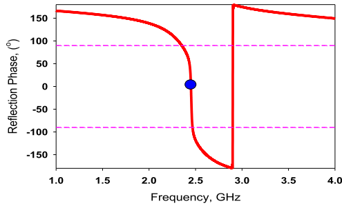
FIGURE 2. Reflection phase of the AMC unit cell.
