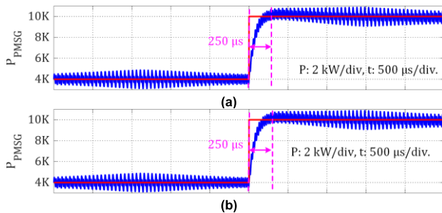
FIGURE 11. Step response for AC input power (a) the proposed converter (Fig. 2), (b) the conventional two-stage converter (Fig. 1(b)).
