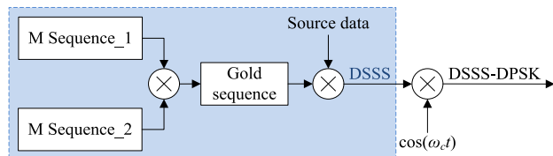
FIGURE 1. Schematic of DSSS-DPSK modulation method.
