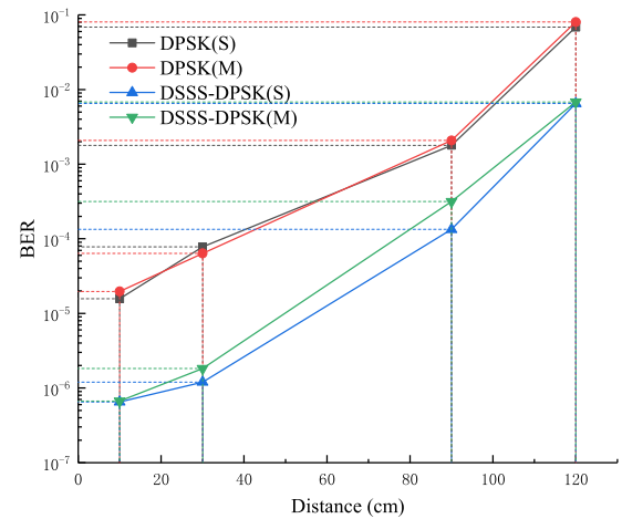
FIGURE 14. SNR performance at different distances when SNR = -5 dB.
