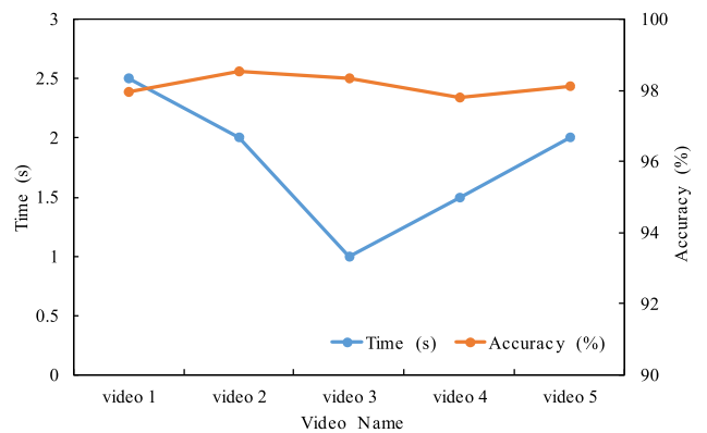
FIGURE 11. Time required for and average accuracy of fire detection for each video.
