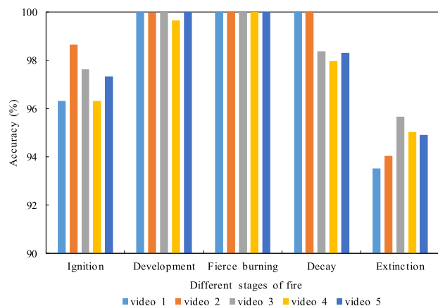
FIGURE 12. Fire detection accuracy in different stages of fire evolution.
