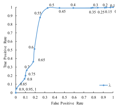
FIGURE 9. ROC curve for different thresholds in dynamic feature extraction.
