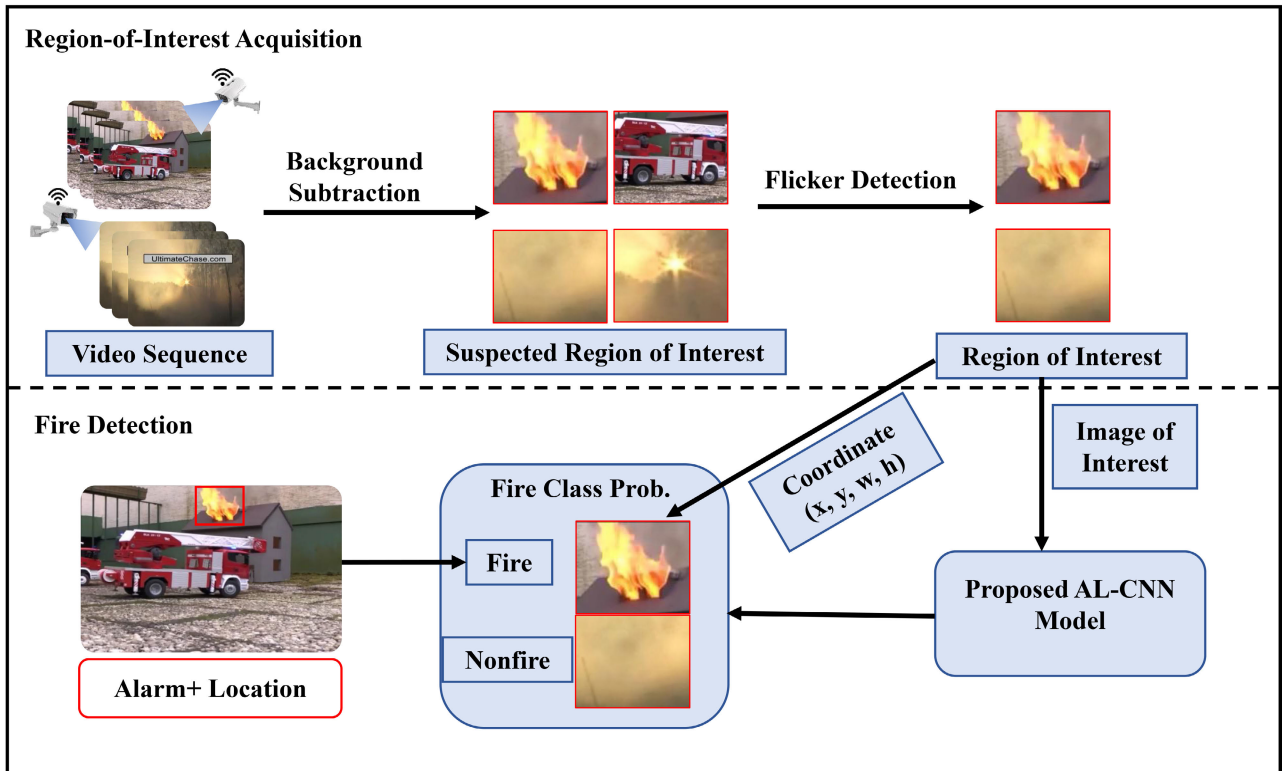
FIGURE 2. The proposed framework for video fire detection exploiting motion-flicker-based dynamic features and deep static features.
