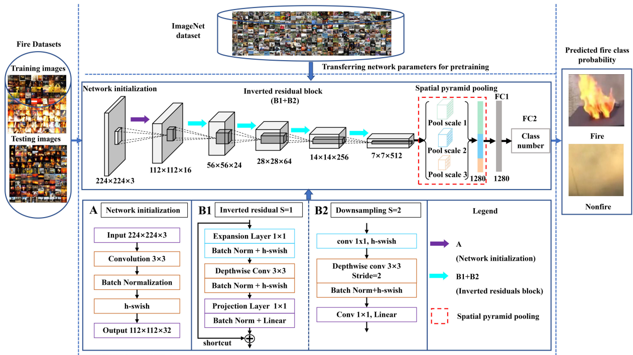
FIGURE 1. Deep static feature extraction framework based on an AL-CNN.
