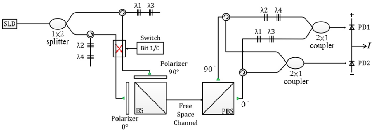
FIGURE 3. FSO communication system using bipolar OCDMA schemes.
