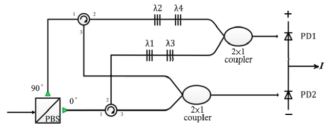
FIGURE 2. Design of the proposed bipolar OCDMA decoder.
