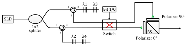
FIGURE 1. Proposed bipolar OCDMA encoder.
