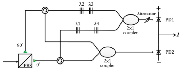
FIGURE 11. Block diagram of FBG decoder 4.
