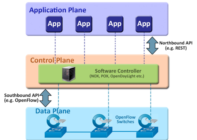
FIGURE 1. SDN architecture.
