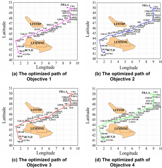
FIGURE 7. The optimized lateral paths of four objectives.
