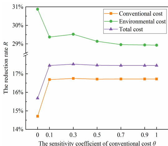
FIGURE 15. The results of the sensitivity study.
