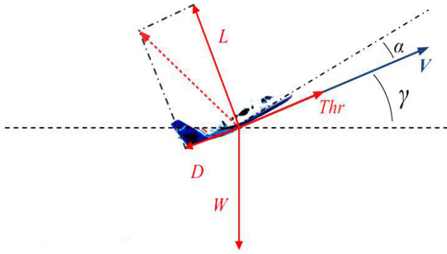
FIGURE 1. Aircraft force.
