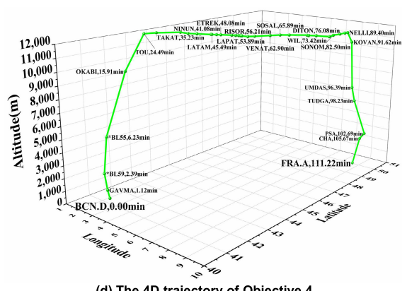
FIGURE 13. The multi-objective 4D optimization trajectories of commercial flight.
