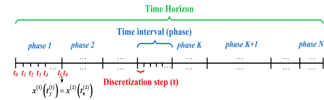
FIGURE 6. Discretization process for vertical profile optimization.
