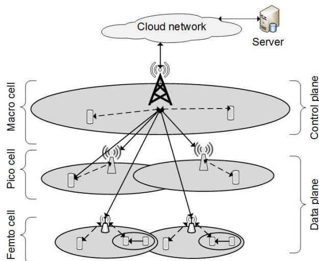
FIGURE 2. 5G architecture. Macro cell, pico cell, and femto cell overlap among themselves. Macro cell handles the control plane and is connected to the cloud network, which consists of the central controller or management node, via backhaul. Dotted lines represent communication in a network cell, such as data transmission from one UE (or network device) to another UE via a relay UE (or service node). Solid lines represent communication between network cells, such as control message exchange between macro cell and small cell BSs (or terminals). For simplicity, BS refers to terminal, UE refers to network device, relay UE refers to service node, and central controller refers to management node.
