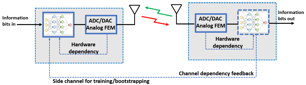
FIGURE 5. End-to-end learning systems adapting to hardware and channels.
