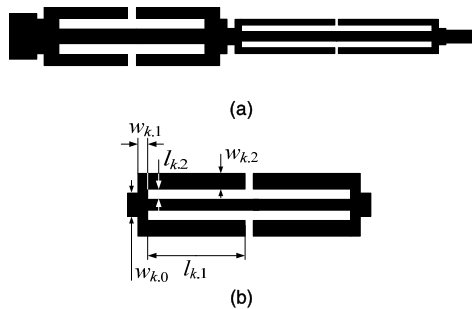
FIGURE 4. CMRC-based compact two-section impedance matching transformer: (a) topology of a two-section structure, (b) compact cell (CMRC).
