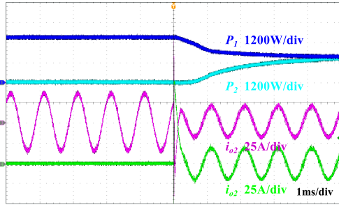
FIGURE 15. Transient performance of hierarchical linear control.
