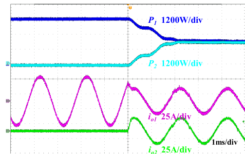
FIGURE 14. Transient performance of proposed scheme.
