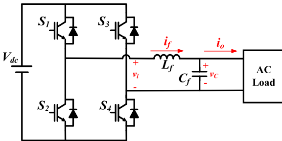
FIGURE 3. Schematic of single-phase LC-filtered VSI.
