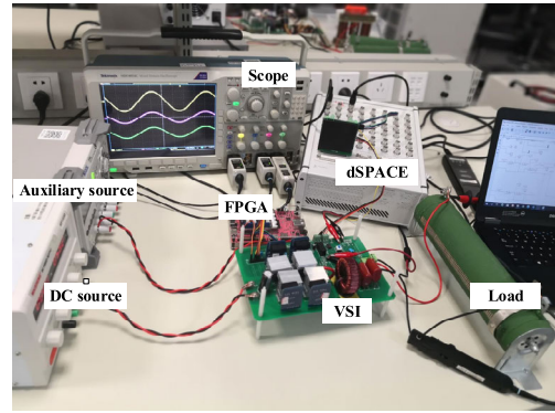
FIGURE 18. Experimental Setup.
