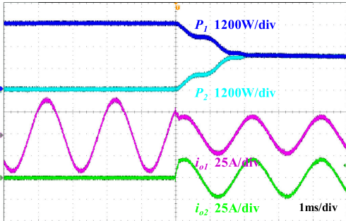
FIGURE 16. Transient performance of two-step FCS MPC.
