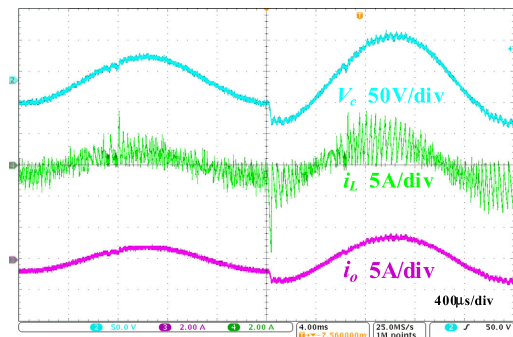
FIGURE 22. Step change performance of proposed FCS-MPC scheme with estimator.
