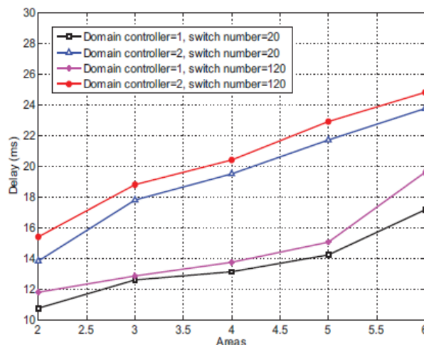
FIGURE 2. Average delay time in Orion [9], [46].
