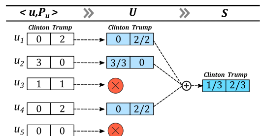
FIGURE 4. Example of how the user polarization algorithm works.
