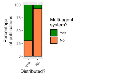
FIGURE 11. Covariance of distributed and multiagent.
