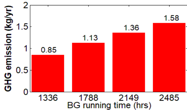
FIGURE 42. GHG emissions vs. BG running time for average solar radiation.
