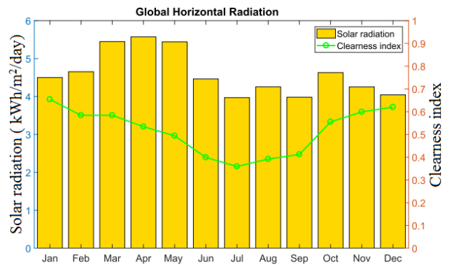
FIGURE 4. Average yearly solar radiation profile in Bangladesh.
