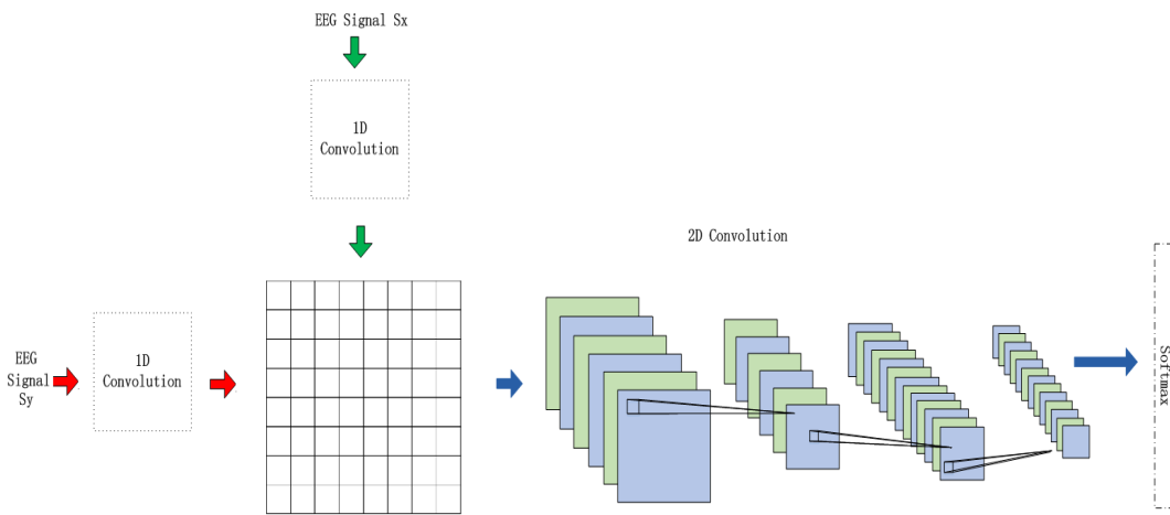
FIGURE 4. The proposed deep learning network architecture.
