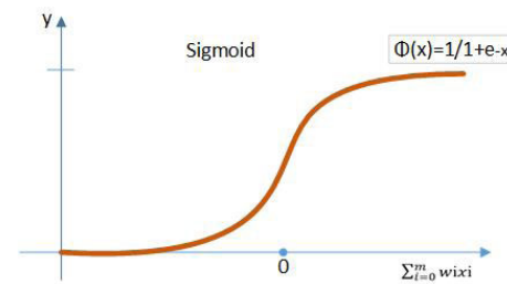
FIGURE 8. Sigmoid AF.
