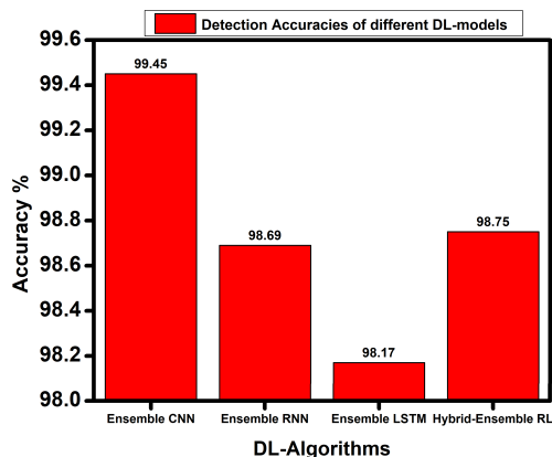
FIGURE 10. Detection accuracies.
