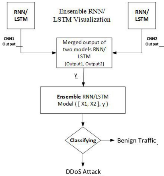
FIGURE 4. Ensemble RNN/LSTM.
