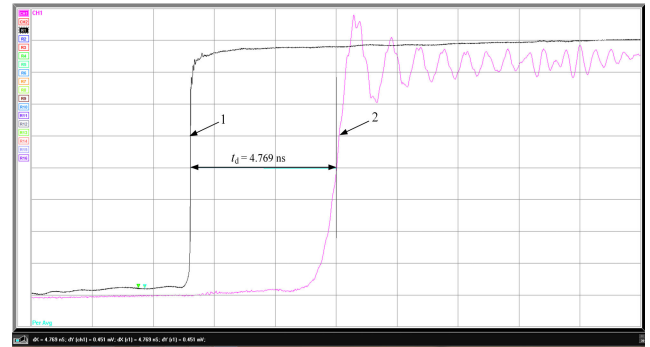
FIGURE 4. An example of signals of input and output pulses of the meander microstrip line, here 1 – pulse at the input of the delay line; 2 – pulse at the output of the delay line, delay time 4.769 ns.
