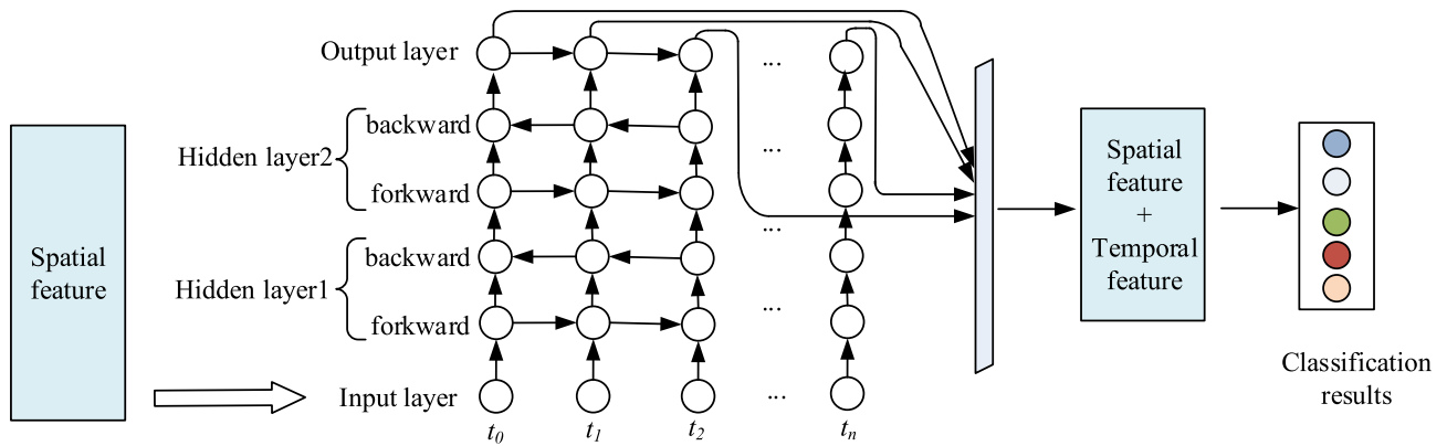
FIGURE 6. Deep hierarchical network structure model.
