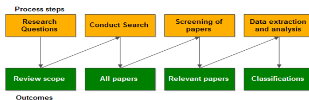
FIGURE 1. Research process.
