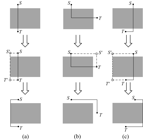
FIGURE 8. Obstacle-avoiding construction by generating virtual vertices.
