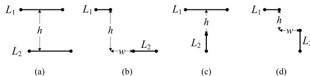
FIGURE 5. Definition of distance between two edges.
