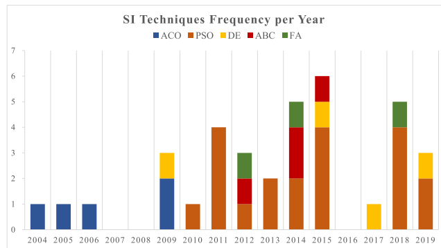
FIGURE 15. Yearly distribution of the SI techniques applied to VLSI routing subproblems in the surveyed works.
