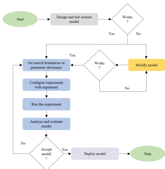
FIGURE 2. Process flow diagram toward the automated optimization of custom CNN hyperparameters using the Talos optimization algorithm.
