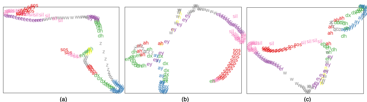
FIGURE 9. T-SNE on “mjd0_si1984” for P1 at epoch 4 (a) & 8 (b) & final epoch (c). Horizontal axis: the 1 st dimension of t-SNE embeddings; vertical axis: the 2 nd dimension of t-SNE embeddings.
