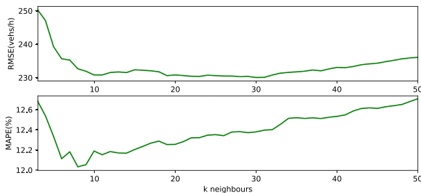
FIGURE 4. The performance of Eu- k NN with different number of neighbors k .
