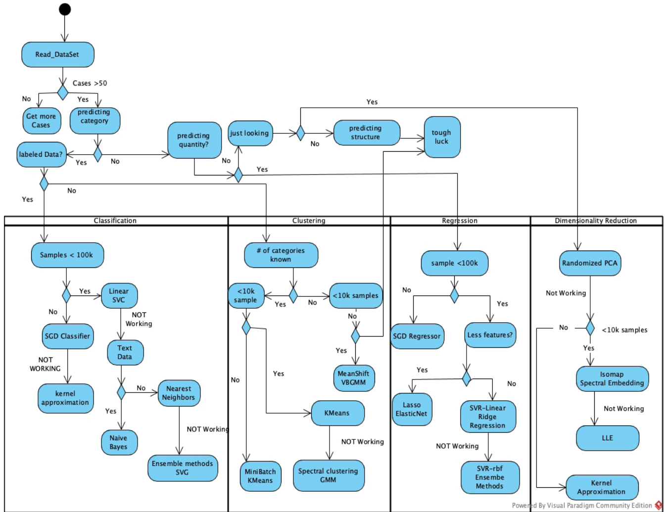
FIGURE 6. Machine algorithm model components.
