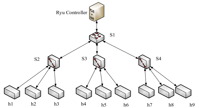
FIGURE 4. Experimental topology.
