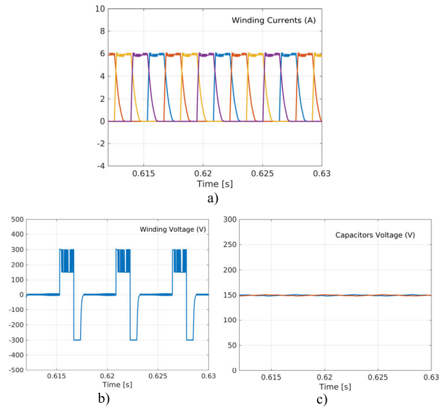
FIGURE 15. Simulation results for the SRM in normal operation for a speed of 1800 rpm: a) Winding currents; b) Applied voltage to winding A; c) Capacitor voltages.
