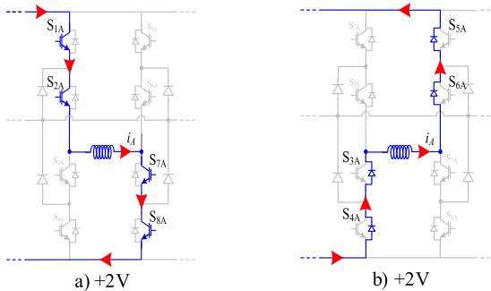
FIGURE 3. Operation modes for the proposed converter in normal operation for the maximum DC voltages.
