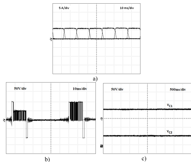
FIGURE 27. Experimental results for the SRM in short-circuit transistor ( S_{1A} ) failure operating at 980 rpm: a) Winding currents; b) Applied voltage to winding A; c) Capacitor voltages.
