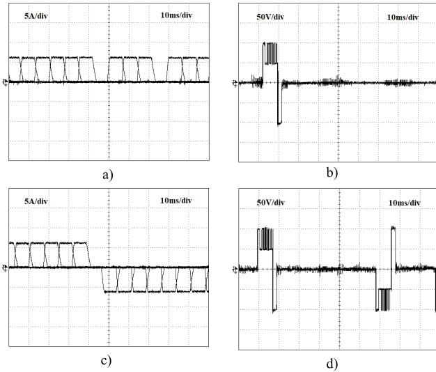
FIGURE 24. Experimental results for the SRM in open-circuit transistor ( S_{2A} ) failure and fault tolerant condition operation at 1870 rpm: a) Winding currents in failure mode; b) Applied voltage to winding A in failure mode; c) Winding currents in fault tolerant operation; d) Applied voltage to winding A in fault tolerant operation.
