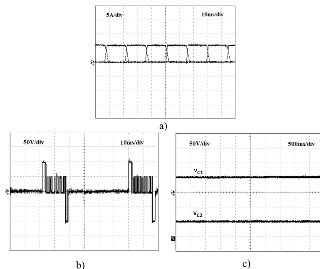
FIGURE 23. Experimental results for the SRM in normal operation for a speed 980 rpm: a) Winding currents; b) Applied voltage to winding A; c) Capacitor voltages.
