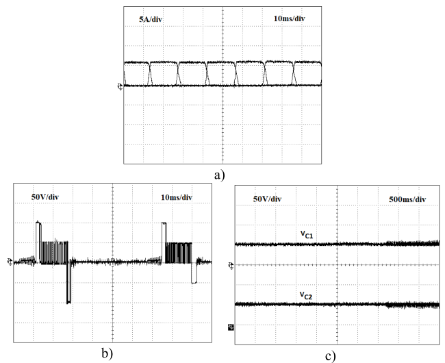
FIGURE 26. Experimental results for the SRM in short-circuit transistor ( S_{2A} ) failure operating at 980 rpm: a) Winding currents; b) Applied voltage to winding A; c) Capacitor voltages.
