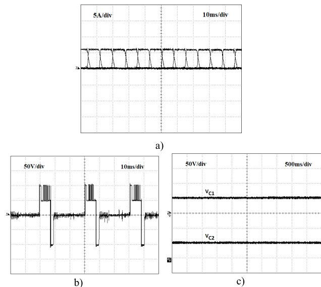
FIGURE 22. Experimental results for the SRM in normal operation for a speed of 1870 rpm: a) Winding currents; b) Applied voltage to winding A; c) Capacitor voltages.
