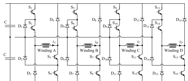
FIGURE 1. Neutral point clamped asymmetrical half-bridge converter (NPC-AHB) topology for SRM drives.
