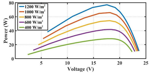
FIGURE 3. Effect of irradiance on PV array performance at T = 25°C.
